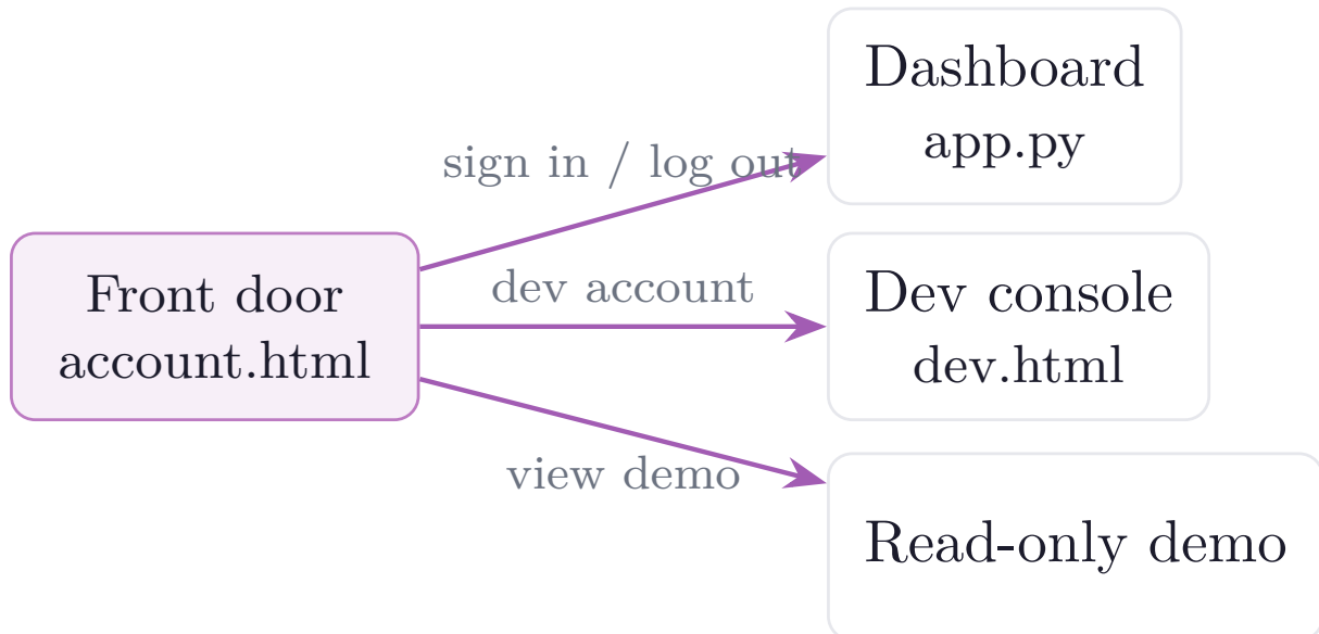
Figure 11: Dashboard page flow. The static front door is the hub for sign-in, the developer console, and the read-only demo.
