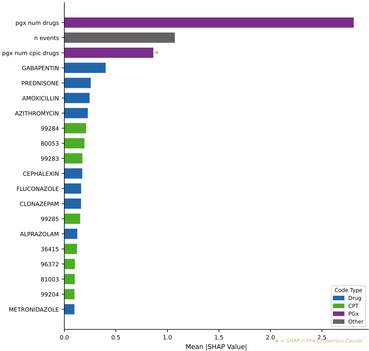
SHAP Feature Importance — Opioid ED, Age 25–44 (Top 20 Consensus-Causal Features, 2019 Holdout)
