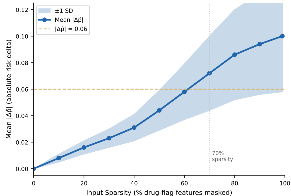
(A) Prediction Error vs. Input Sparsity (1,000 bootstrap trials; 2019 holdout)
