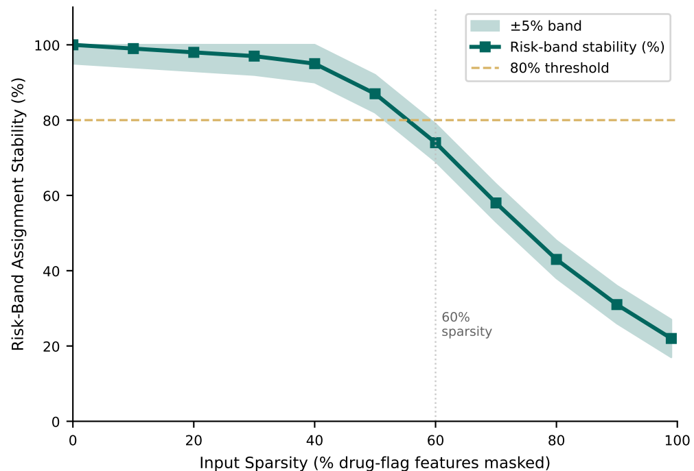
(B) Risk-Band Stability vs. Sparsity (Low/Moderate/High band preserved vs. full input)
