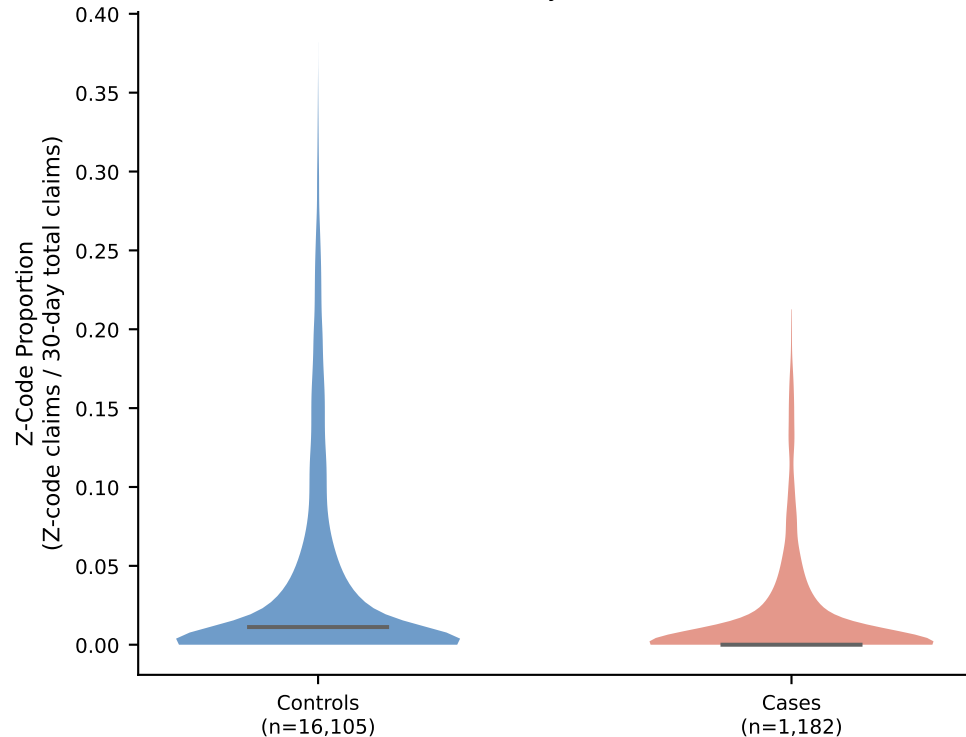
(A) Z-Code Proportion by ADE Status (Mann-Whitney U, P < 0.001 )
