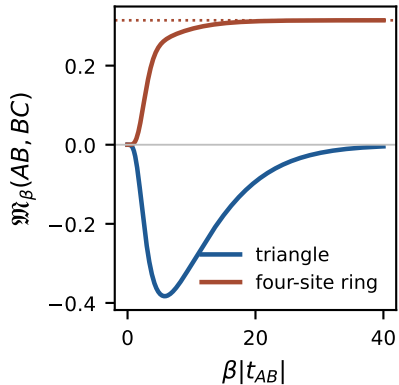
(a) Thermal crossover
