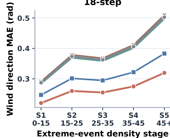
(f) Penmanshiel - Wind direction 18-step
