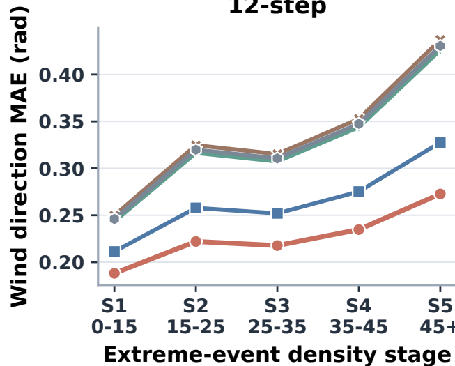
(e) Penmanshiel - Wind direction 12-step
