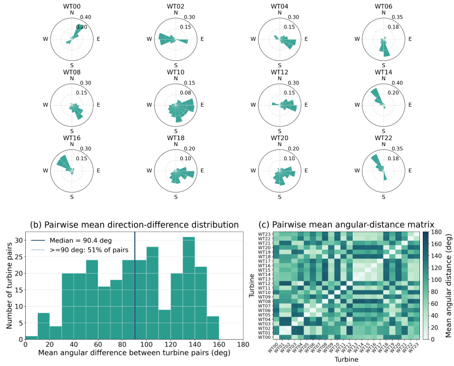
Figure 3: Turbine-specific wind-direction distributions and all-pair angular differences among 24 turbines.
