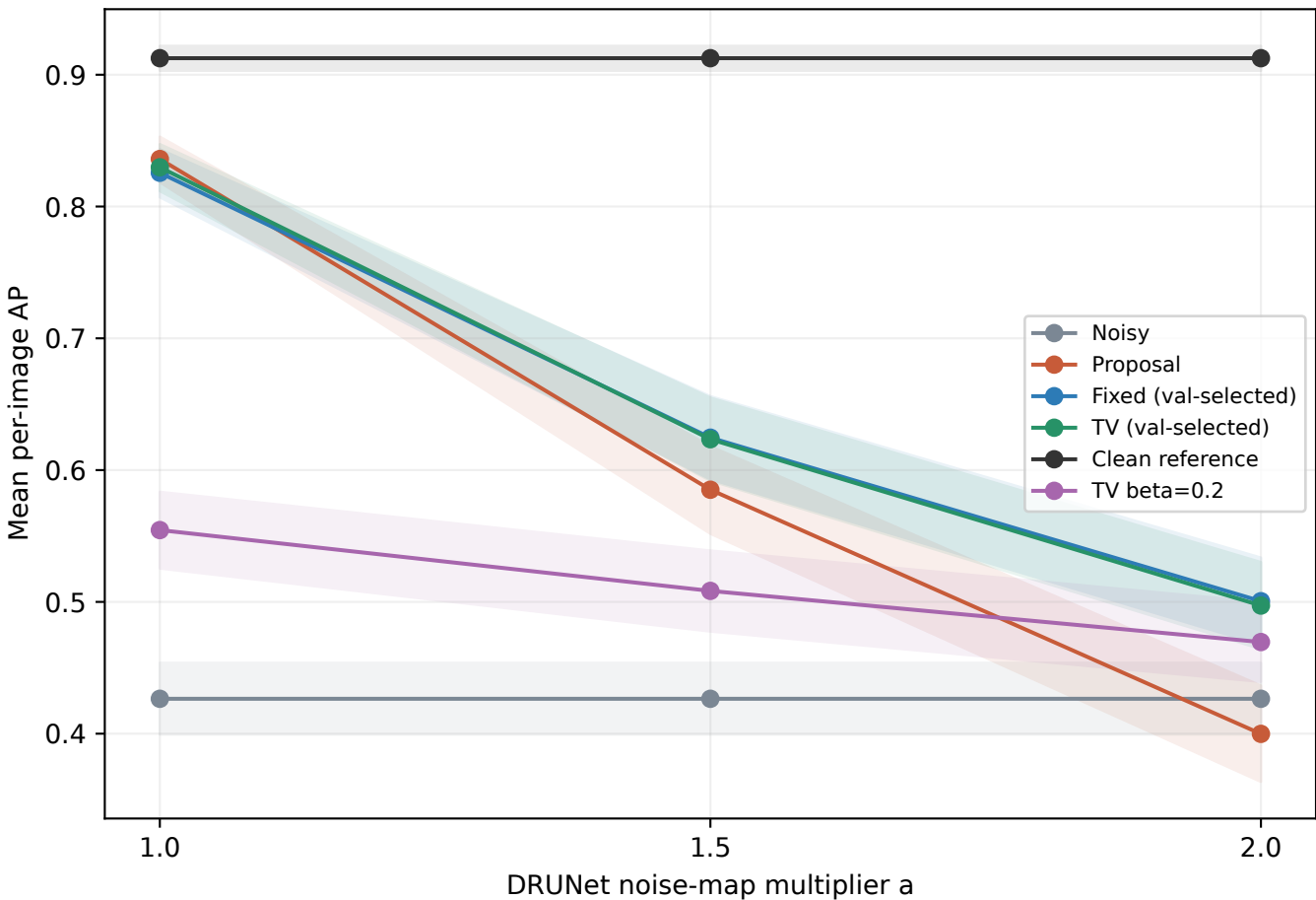
Test robustness (geometry bootstrap 95% CI)
