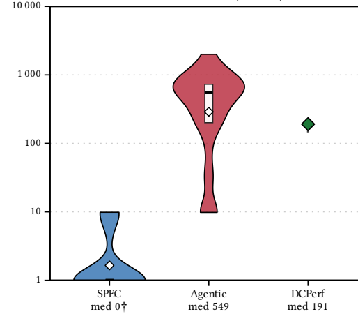
Context switches (/CPU-s)
