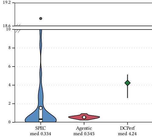
L2-load MPKI
