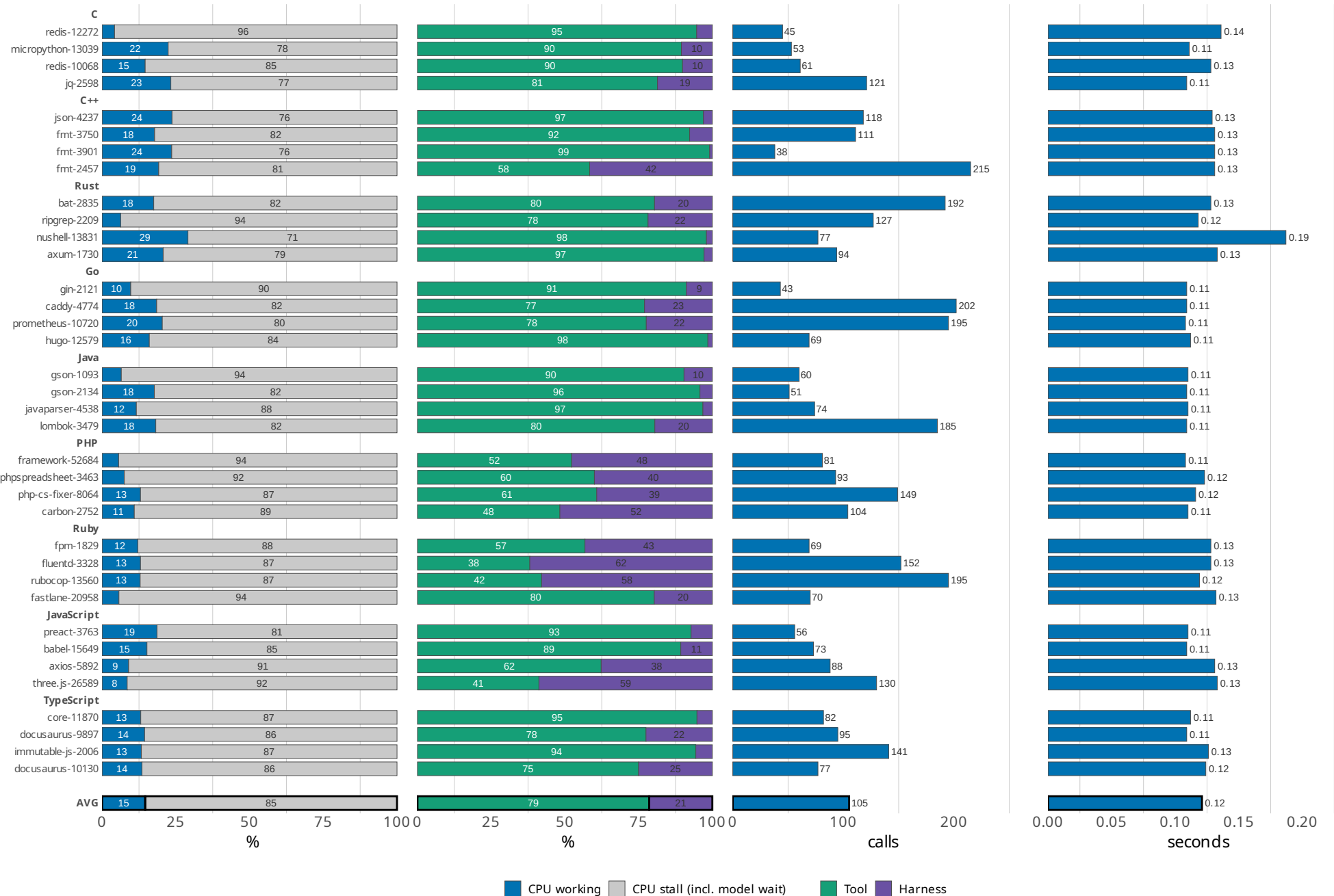
(a) CPU working vs. stall
