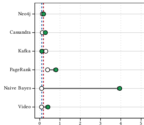
LLC MPKI
