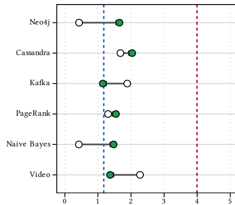
Branch MPKI
