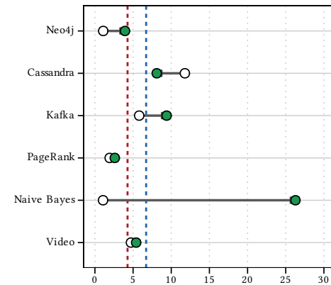
L1D-load MPKI
