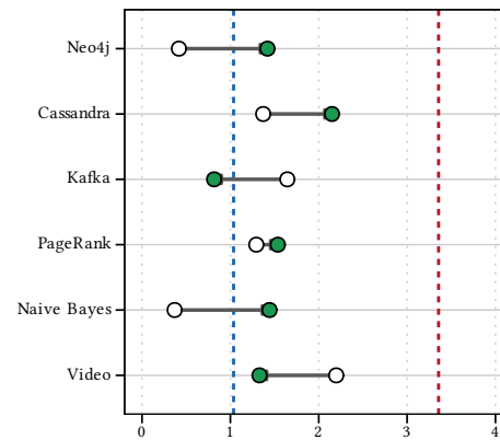
Branch-direction MPKI
