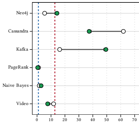
L1I MPKI (code-read)
