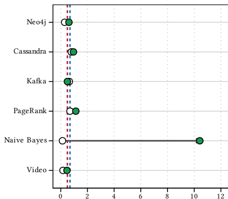
L2-load MPKI
