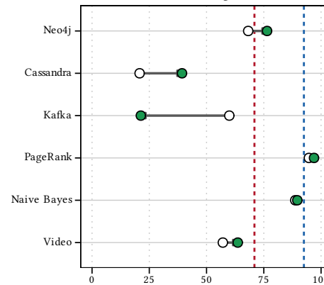
DSB coverage (%)
