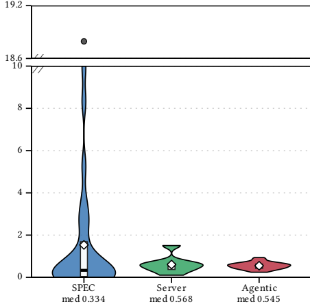
L2-load MPKI
