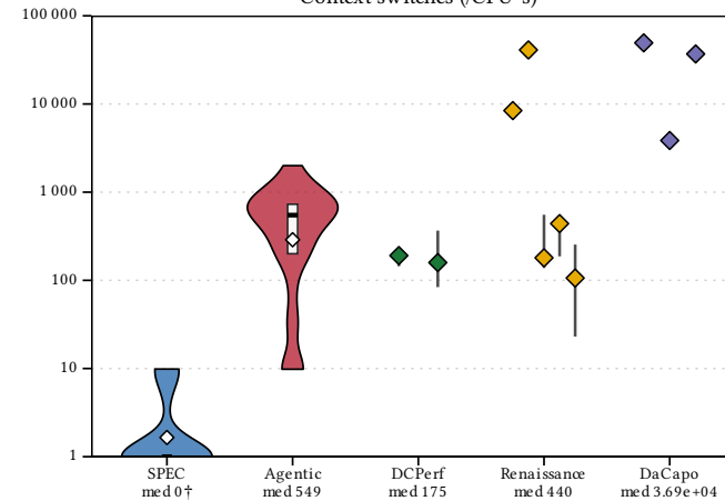
Context switches (/CPU-s)
