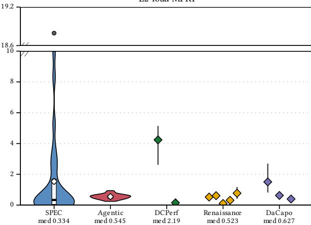
L2-load MPKI
