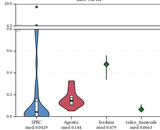
LLC MPKI
