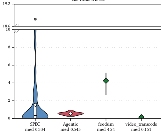
L2-load MPKI
