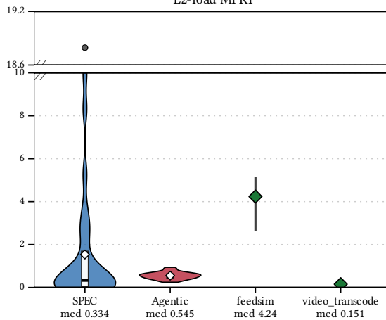
L2-load MPKI
