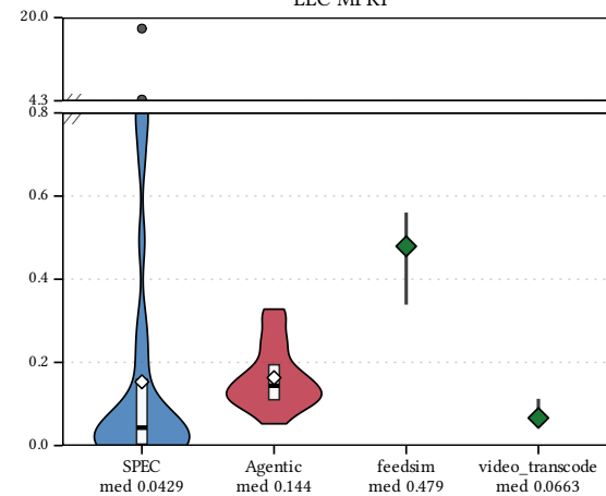
LLC MPKI
