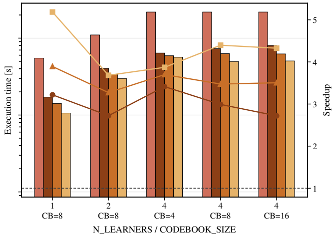
BERT-base
