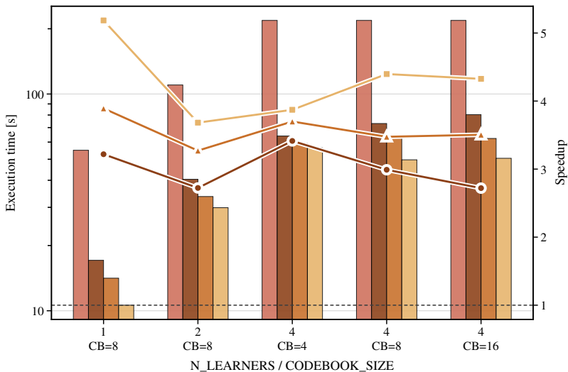
BERT-base
