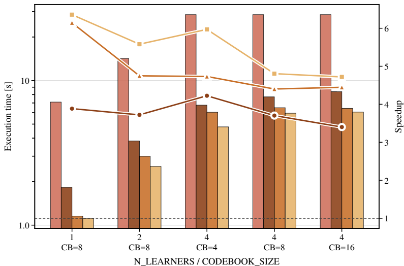
BERT-base
