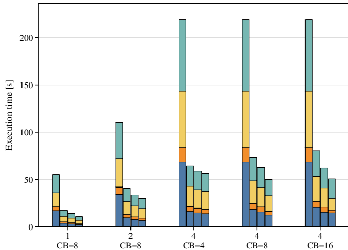
BERT-base
