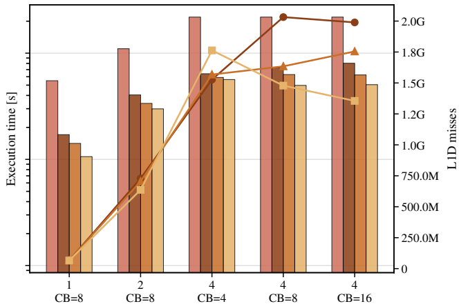
BERT-base
