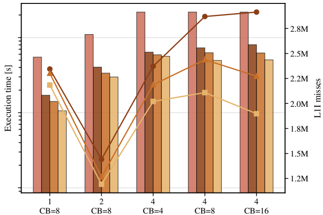
BERT-base
