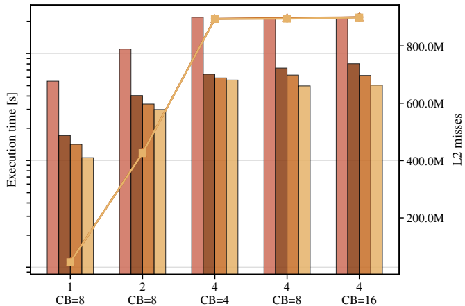
BERT-base
