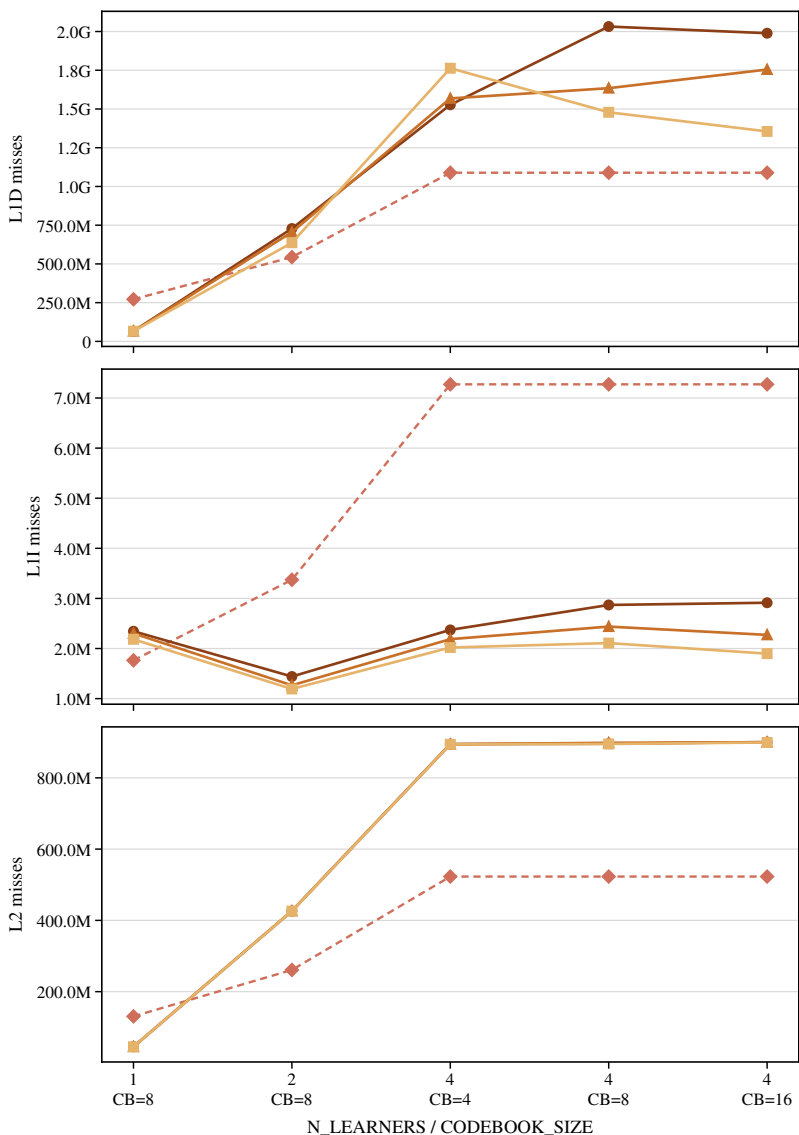
BERT-base
