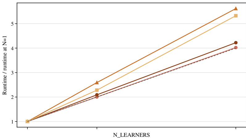
BERT-base
