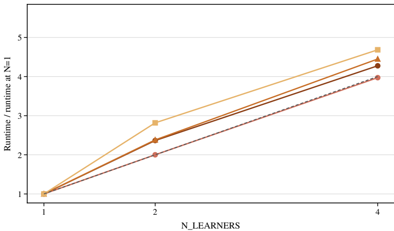
BERT-base
