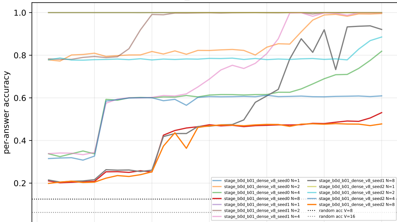
dense_capped: accuracy
