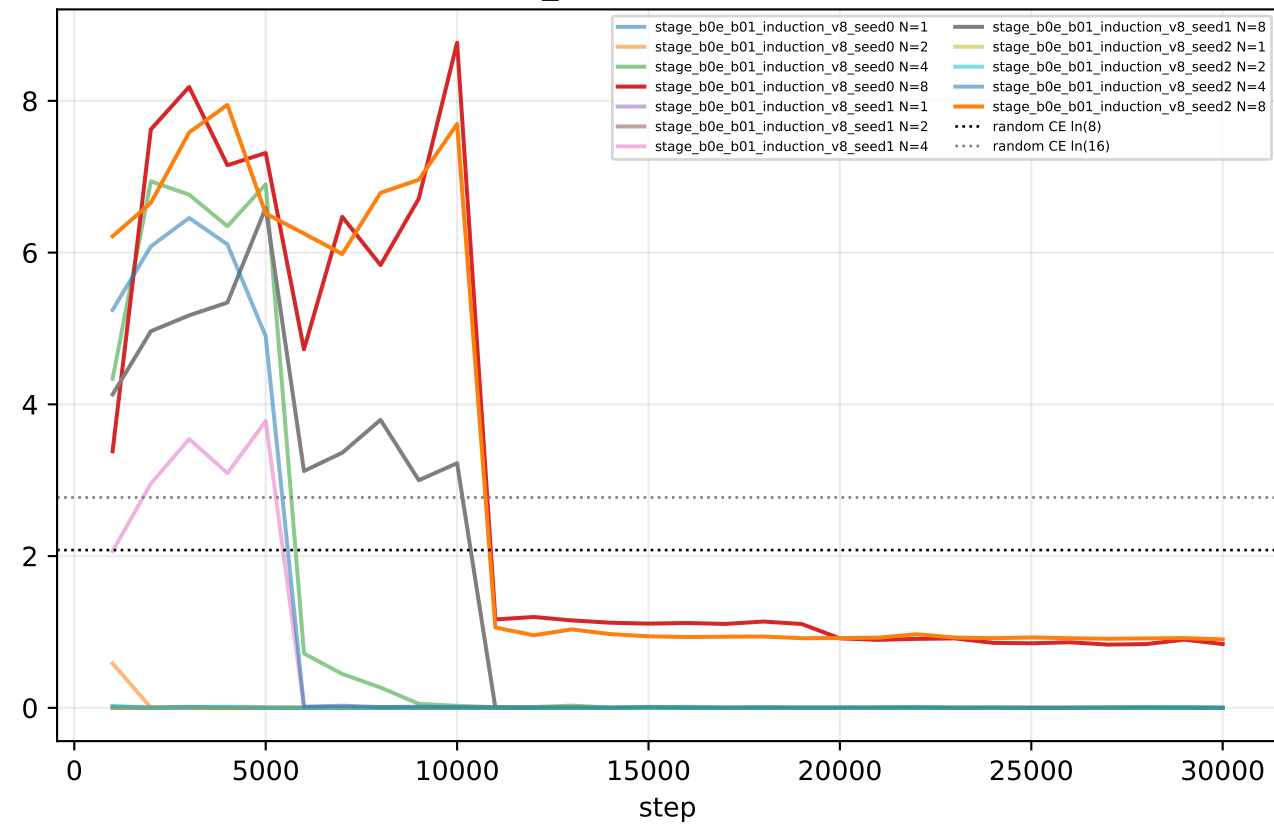
single_query: cross-entropy
