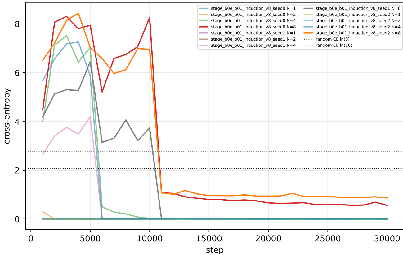
induction_capped: cross-entropy
