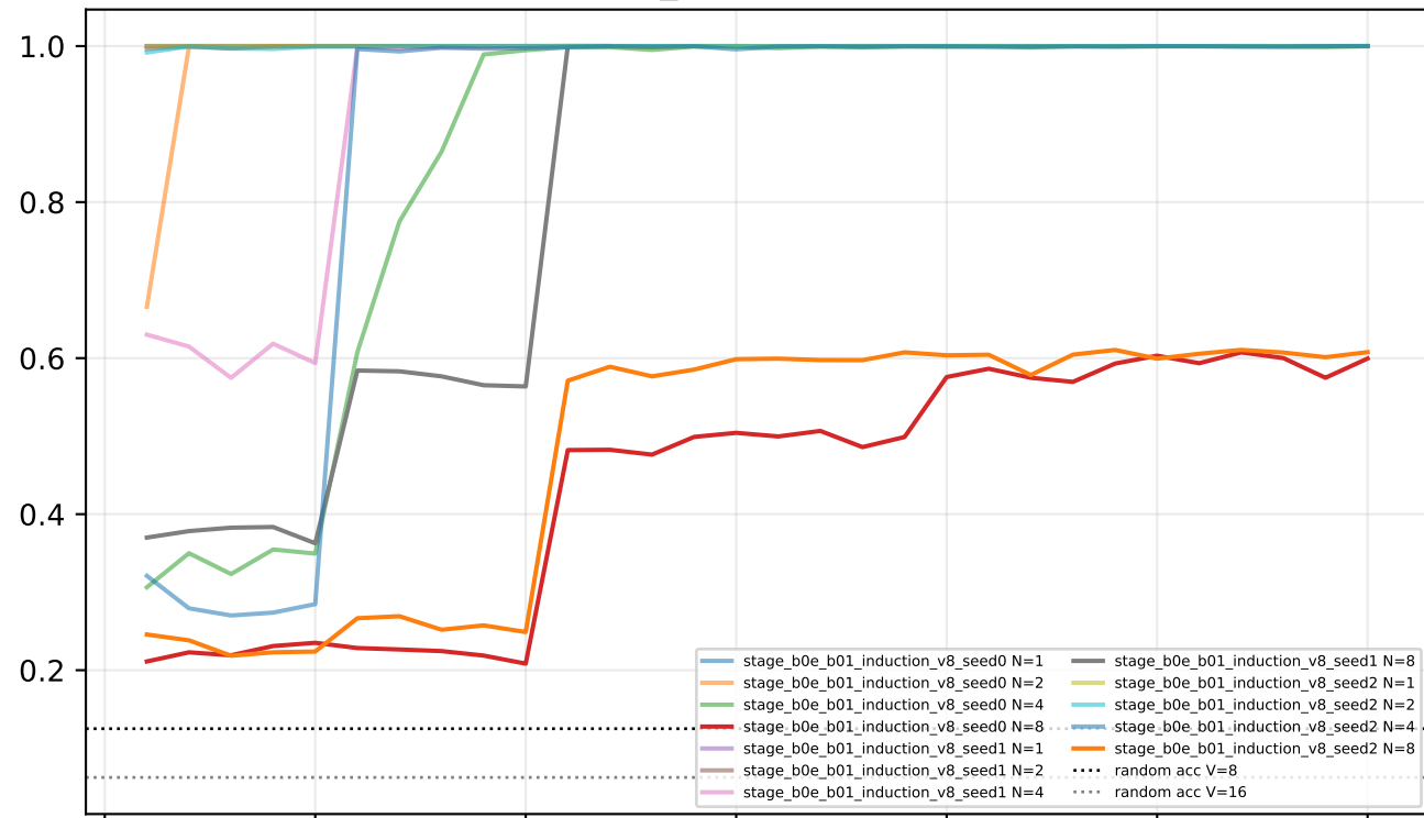
single_query: accuracy
