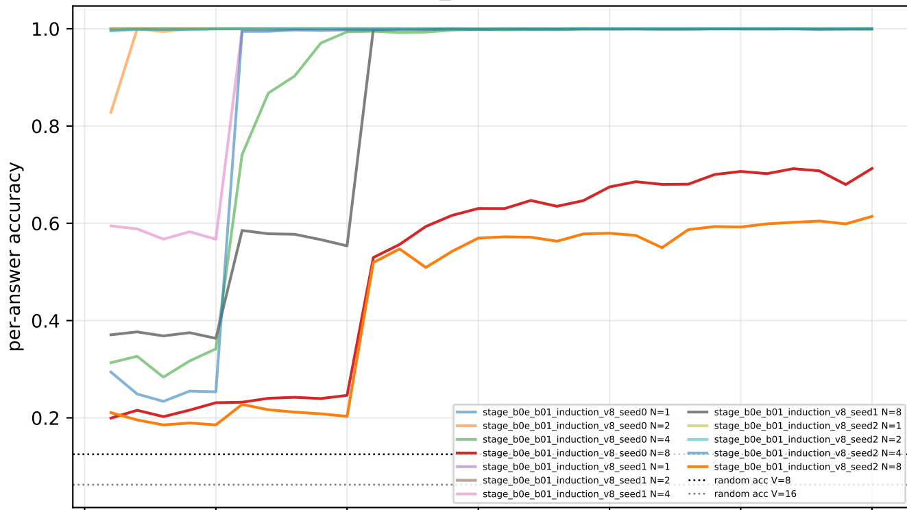
induction_capped: accuracy
