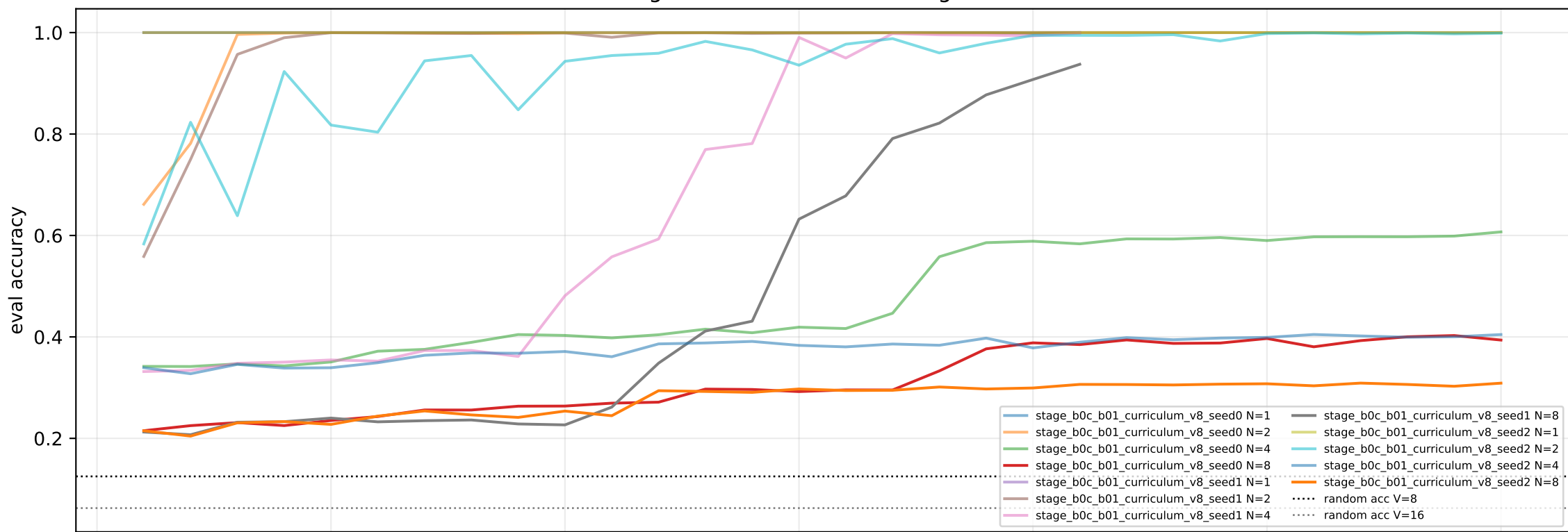
Stage B0C curriculum learning curves
