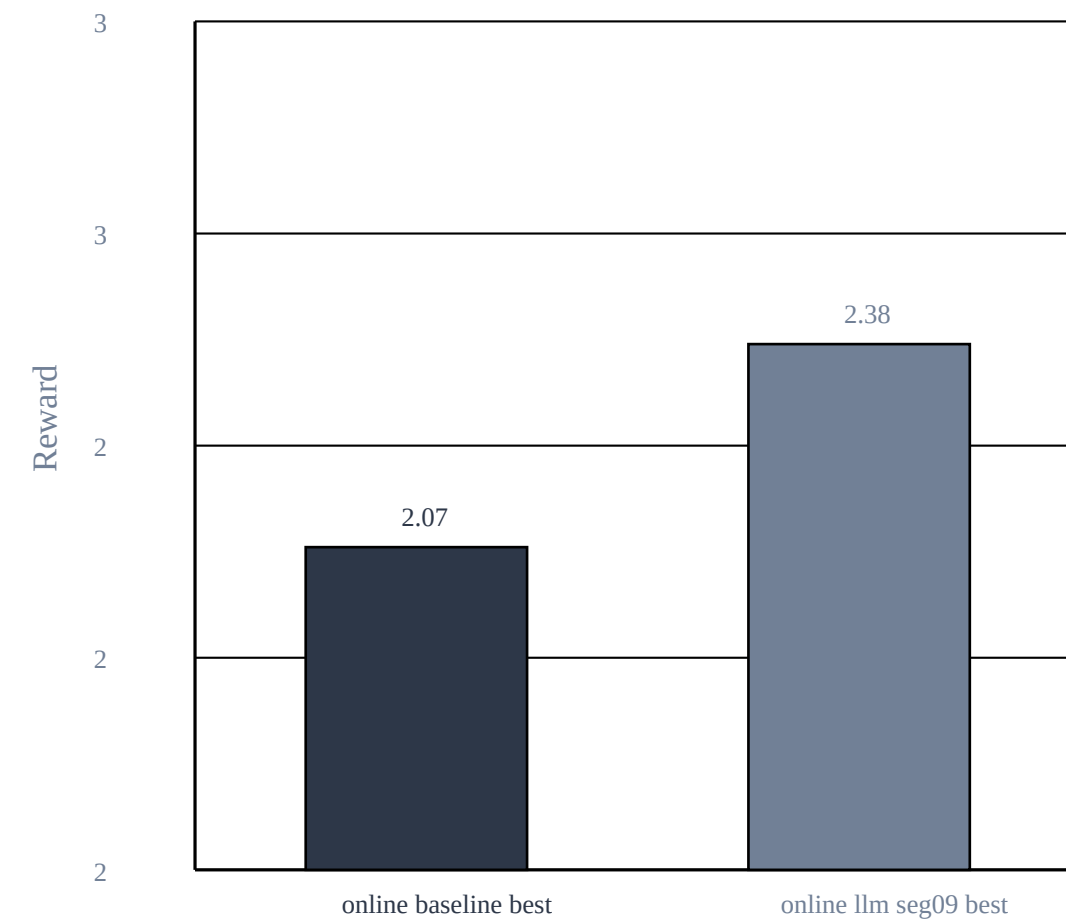
Mean Success Reward
