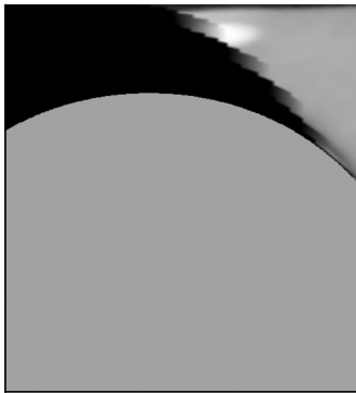
sample 0
