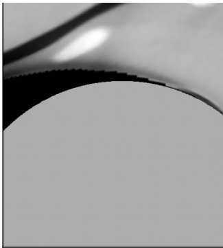
sample 19
