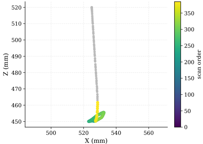
EE trajectory, side (X-Z)
