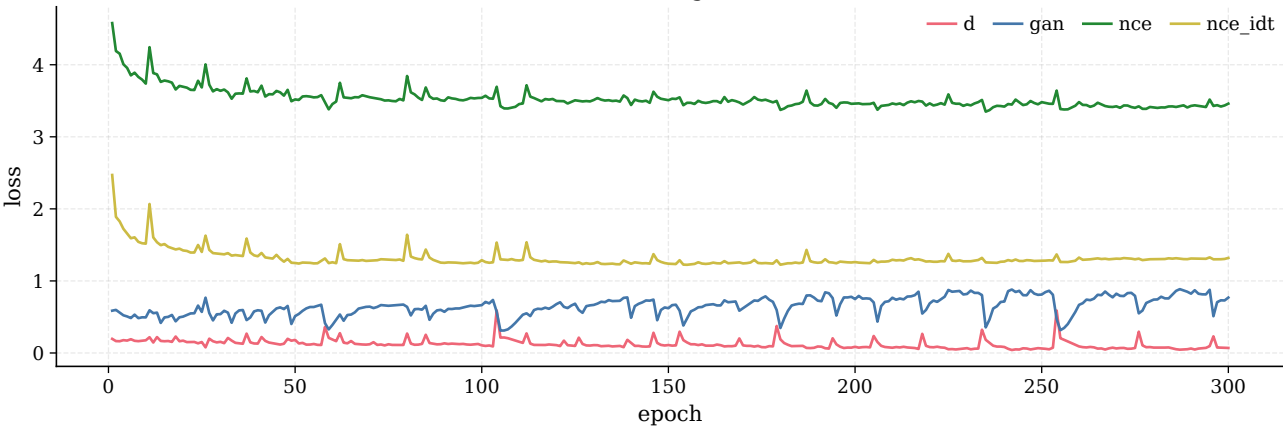
CUT training losses
