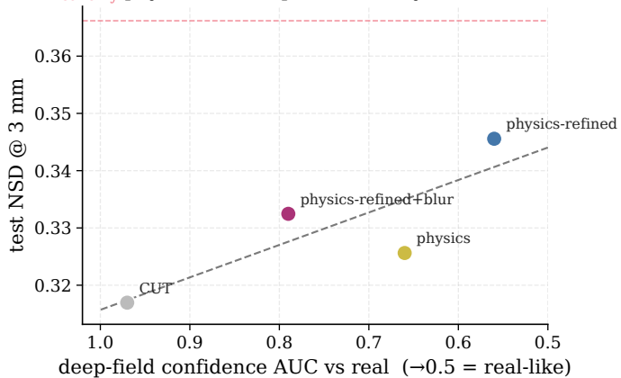
(b) physics realism predicts utility ( r = -0.83 )
