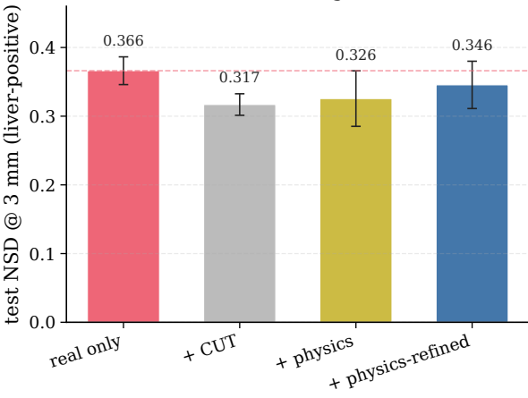
(a) downstream segmentation
