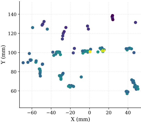
probe positions, top (X-Y)
