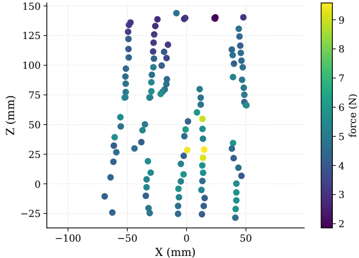
probe positions, side (X-Z)
