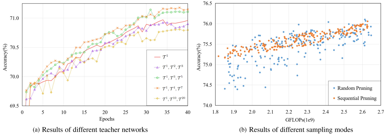
Fig. 5. Ablation studies on distillation teachers and random selection. a) The impact of choosing different large networks as teacher networks on knowledge distillation; b) Accuracy/FLOPs of the 200 sampled subnets on ResNet-50.
