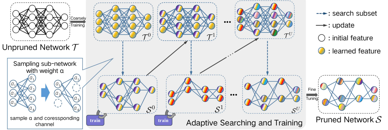
Fig. 2. Detailed illustration of the adaptive search-and-training method. First, we sample compact subnets of the target network based on weight \alpha . Second, we search, train, and map the subnets to the target network. Note that such a search-train-map process will be iterated until the sampled subnets converge. The best performing subnetwork is finally fine-tuned into the output pruned network.
