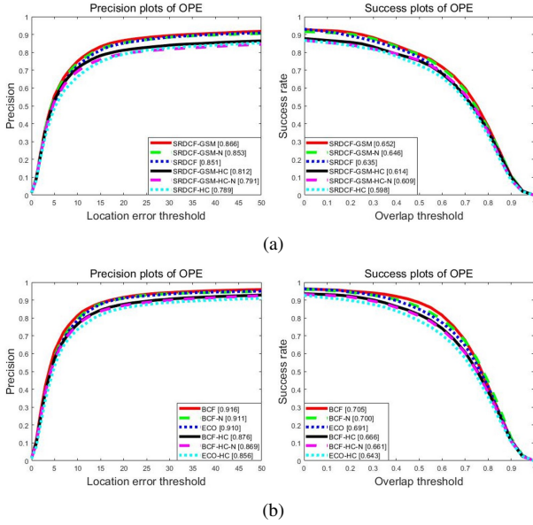
Fig. 9: The success and precision scores of each component of our model on OTB-2015 with hand-crafted features and deep features. (a) Area under curve (AUC) scores based on SRDCF, (b) Area under curve (AUC) scores based on ECO.
