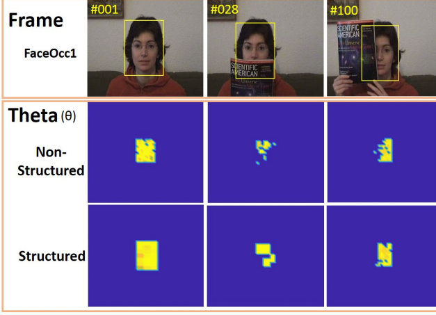
Fig. 3: Comparison of positive scaling variable ( \theta ) with GSM (middle row) and Structured GSM (bottom row) at different times. The distribution of \theta parameters in GSM are more random and has less spatial correlation among the CF coefficients than Structured GSM.
