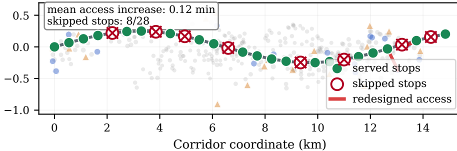
Access reassignment after stop-skipping
