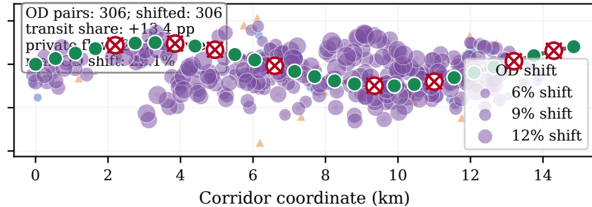
Private-to-transit shift by OD pair
