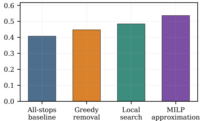
Runtime (s)
