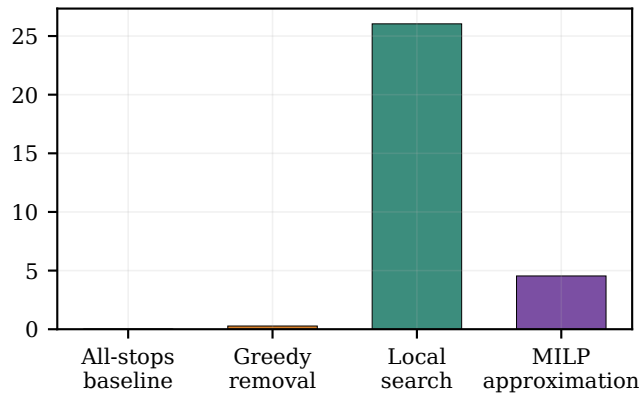
Runtime (s)
