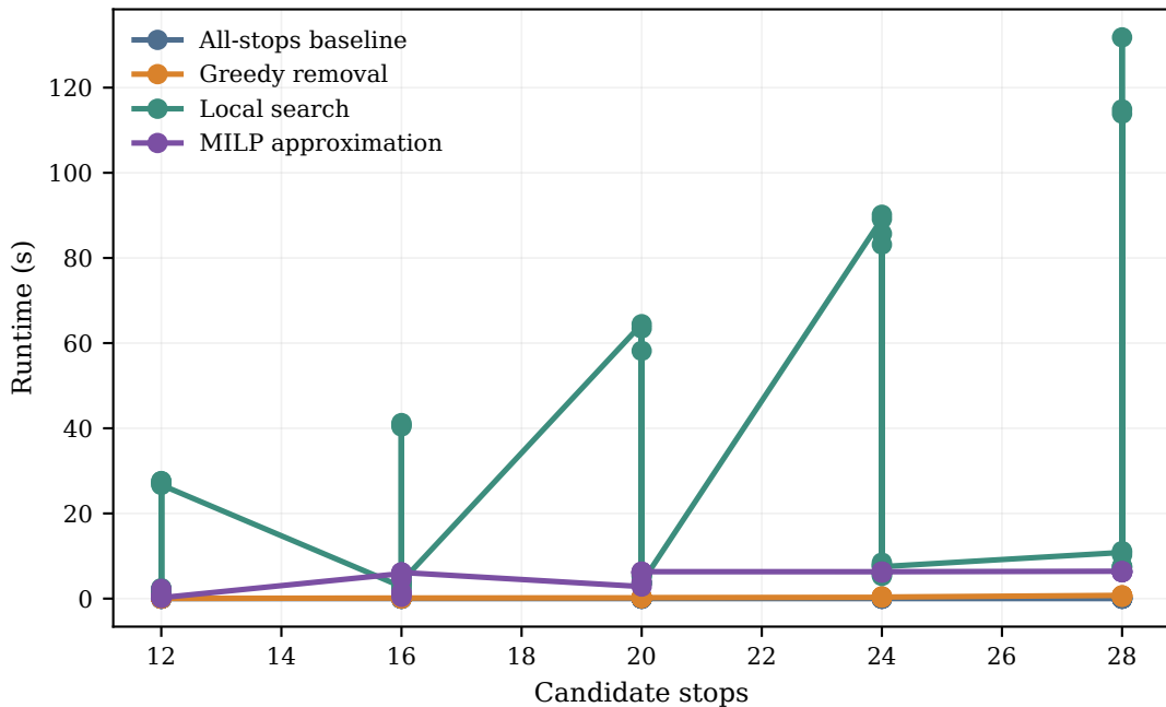
Computational scaling
