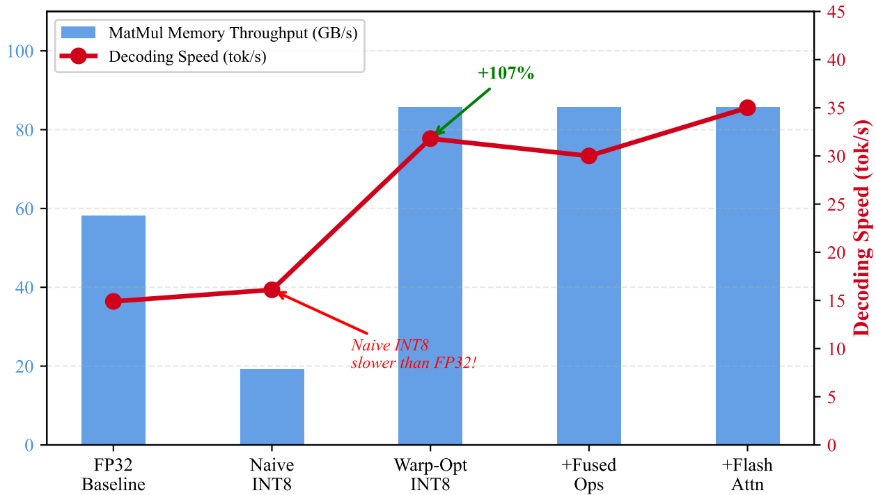
MatMul Memory Throughput (GB/s)
