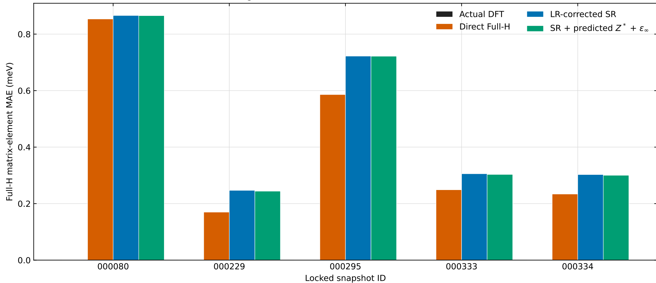
Configuration-resolved held-out Hamiltonian error
