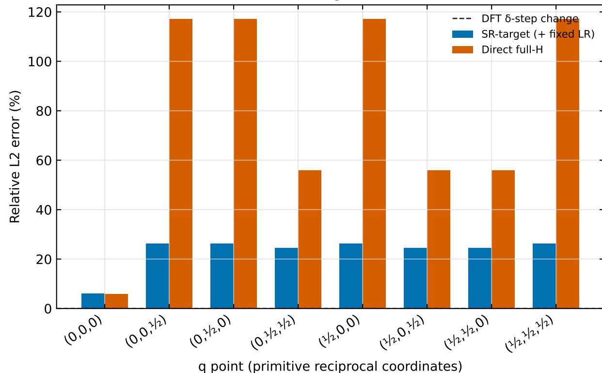
EPC error against DFT
