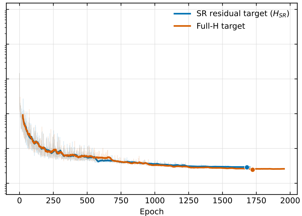
Validation loss
