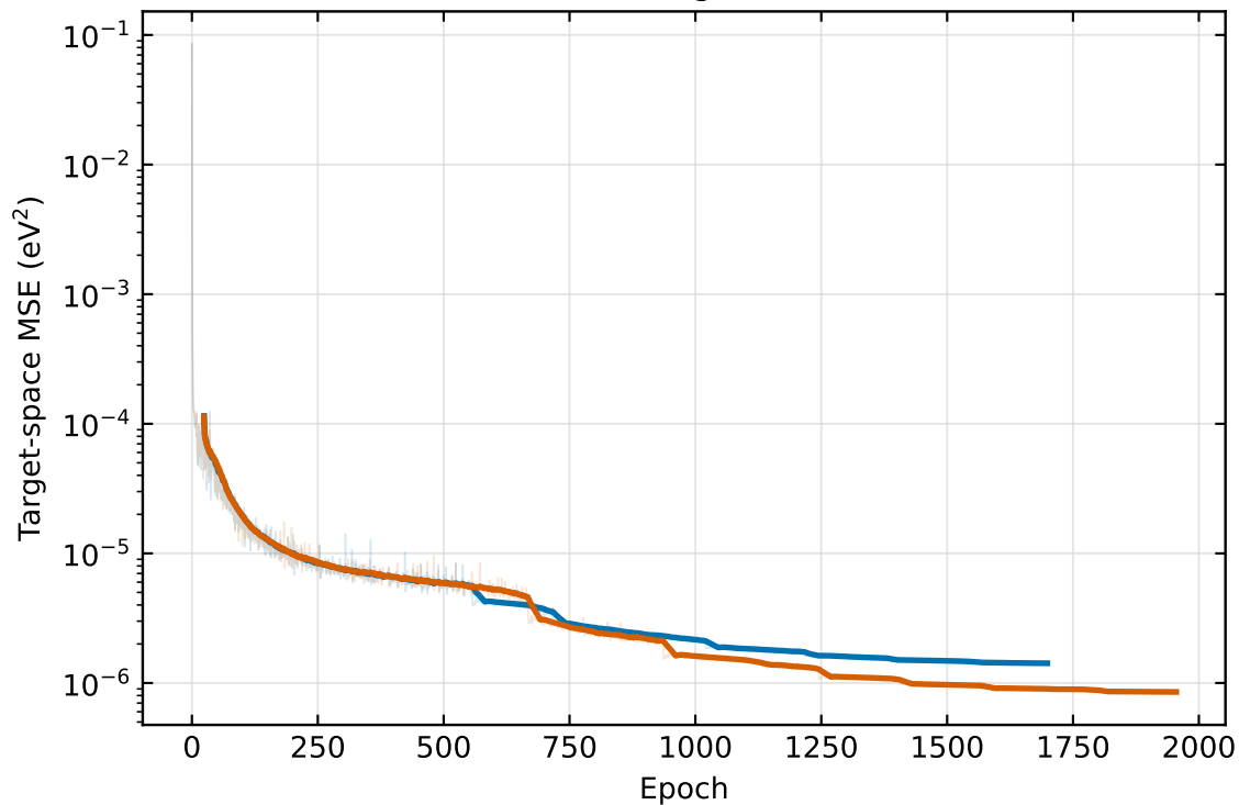
Training loss
