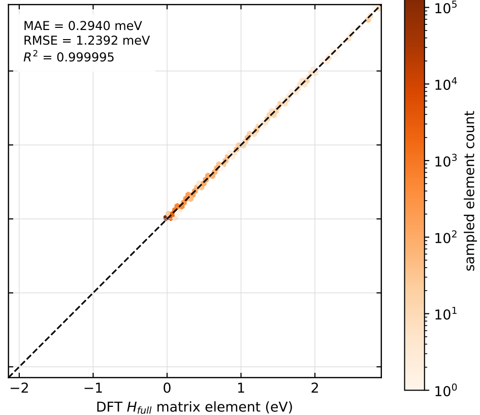
Direct full-H
