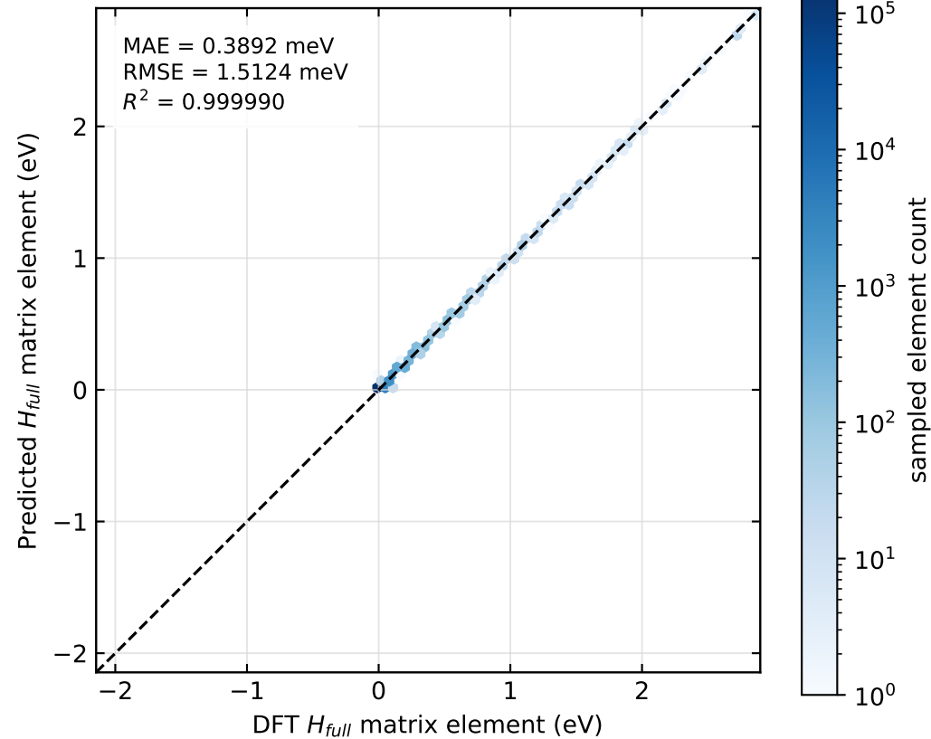
LR-corrected SR
