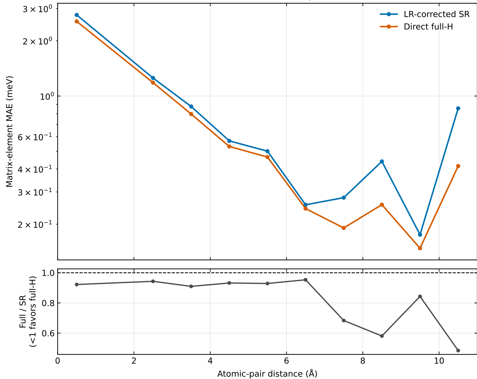
Held-out error versus atomic-pair distance
