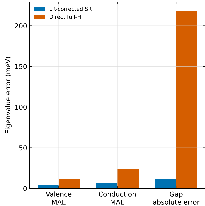
Near-gap errors DFT gap = 4.122 eV
