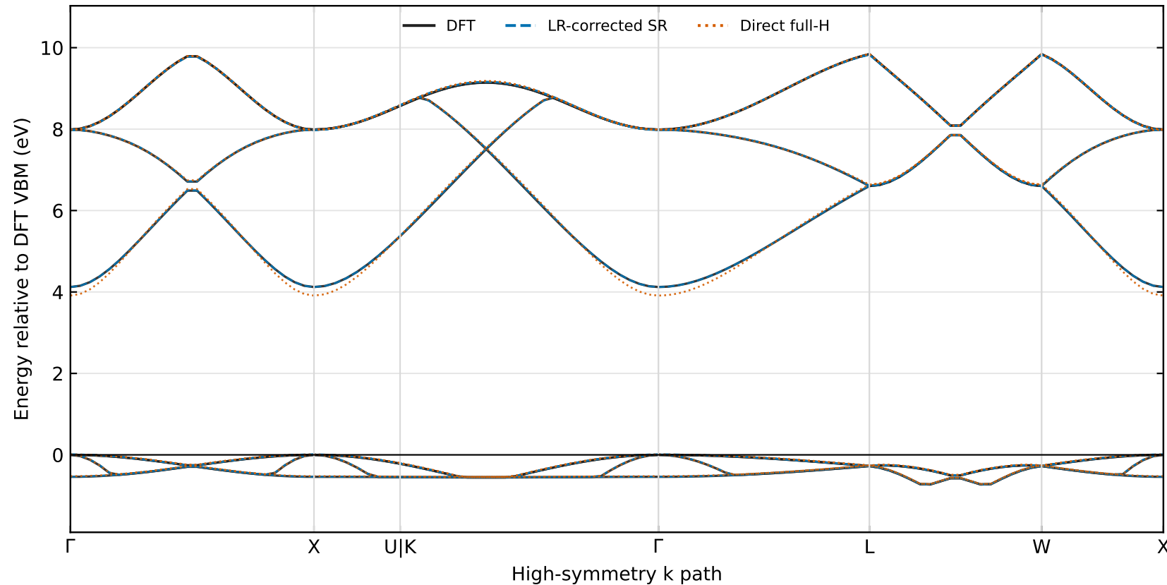
Held-out equilibrium 2\times 2\times 2 MgO bands
