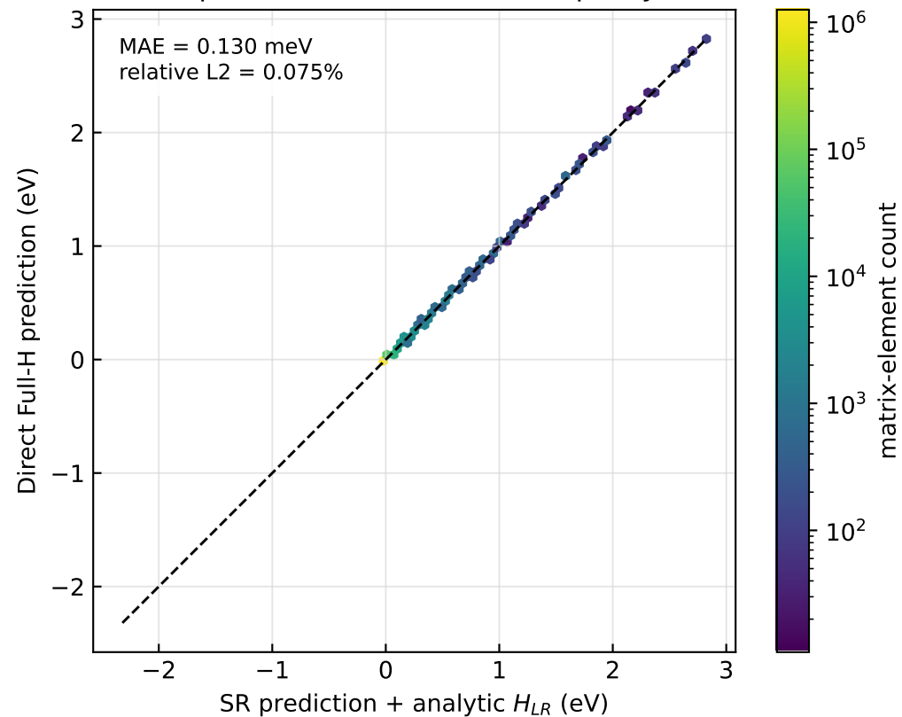
Equilibrium model-to-model parity
