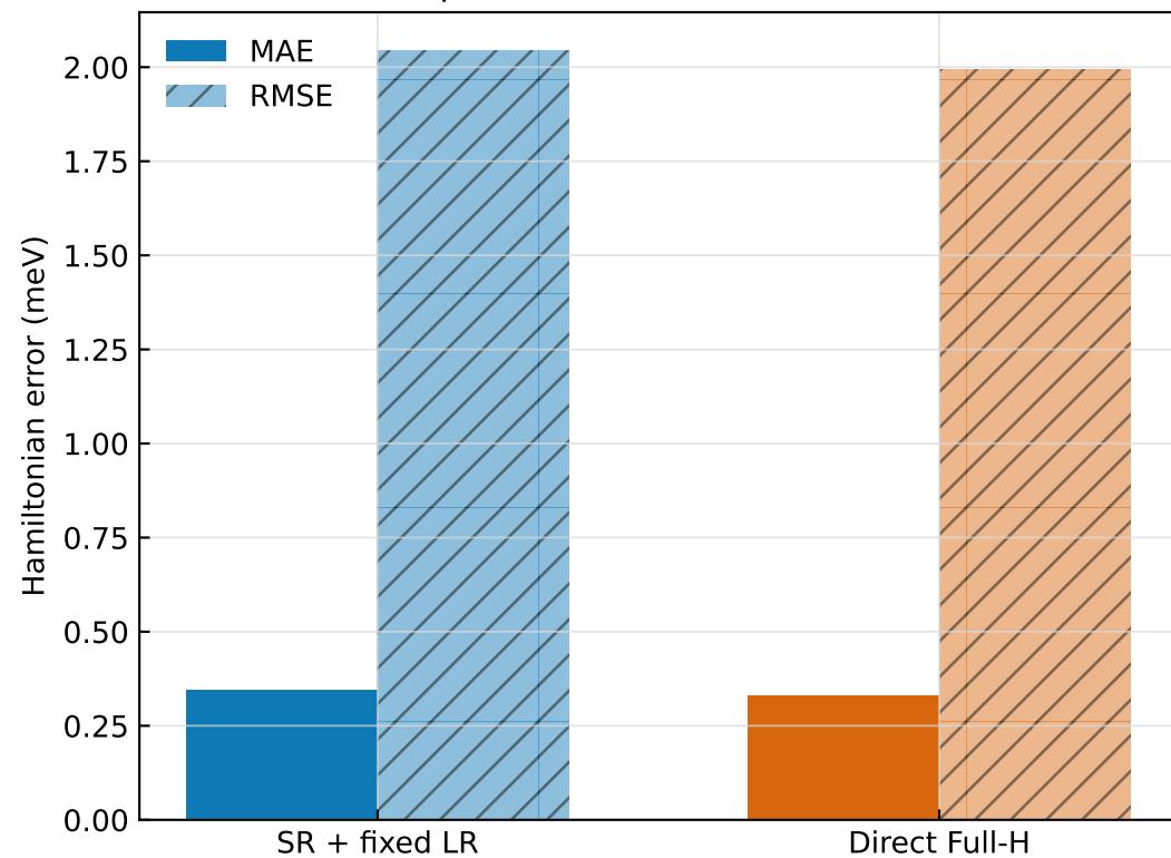
Equilibrium error versus DFT
