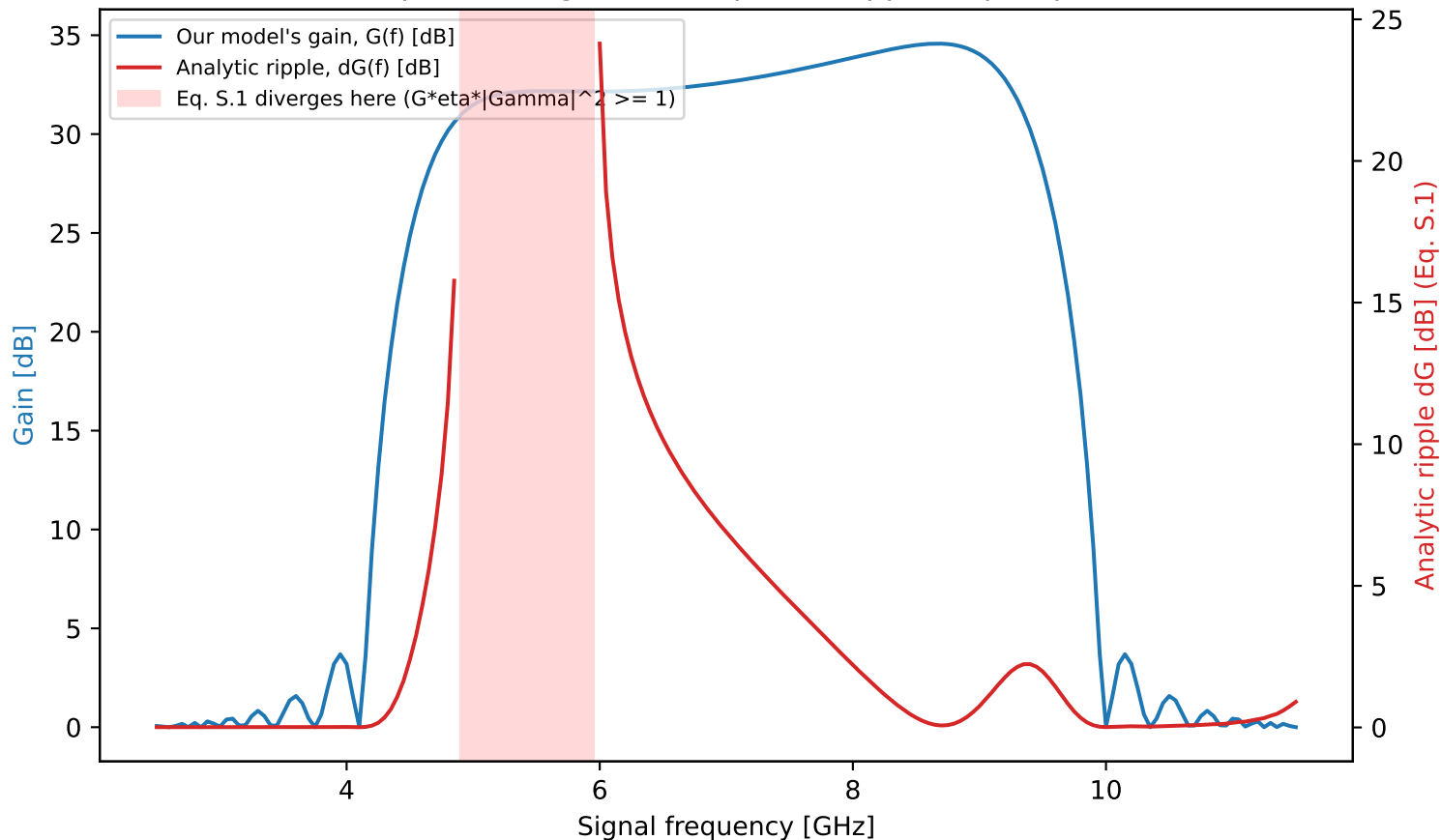
Our device: predicted gain and Eq. (S.1) ripple at pump=14.1 GHz
