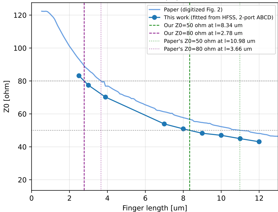
Our HFSS stack vs. the paper's own curve
