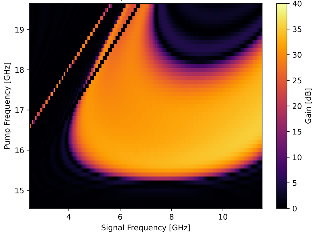
Gain dome (impedance-matched device)
