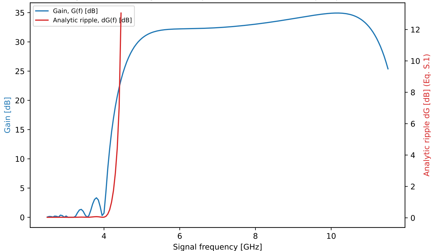
Redesigned structure: gain and Eq. (S.1) domain check at pump=16.0 GHz
