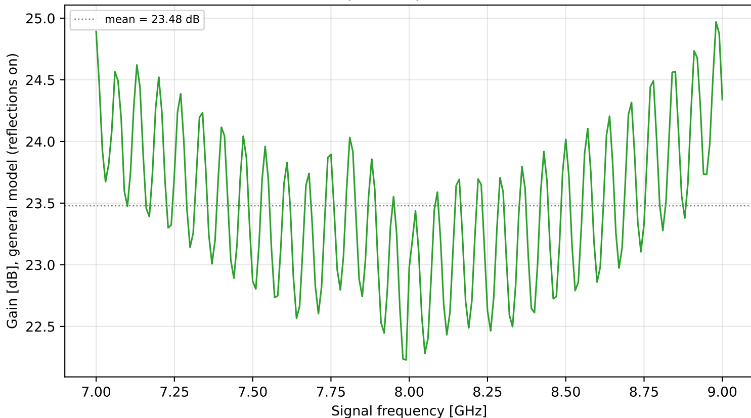
Reflection-enabled numerical model: gain ripple observed peak-to-peak = 2.742 dB
